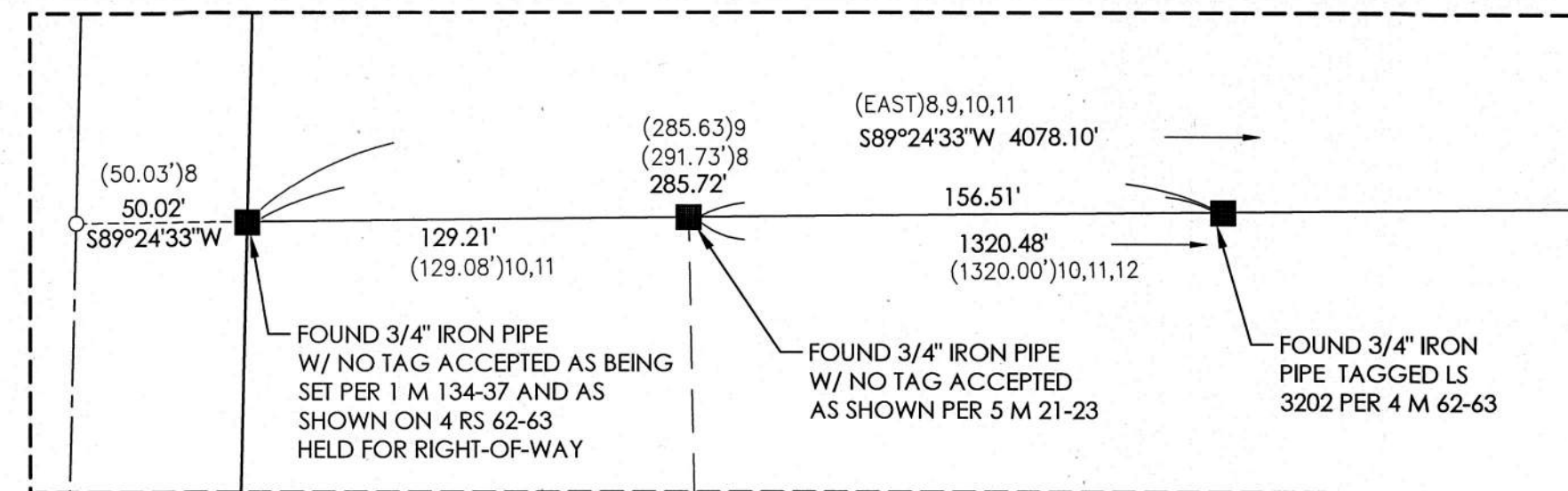
DETAIL 4 1"=50'
