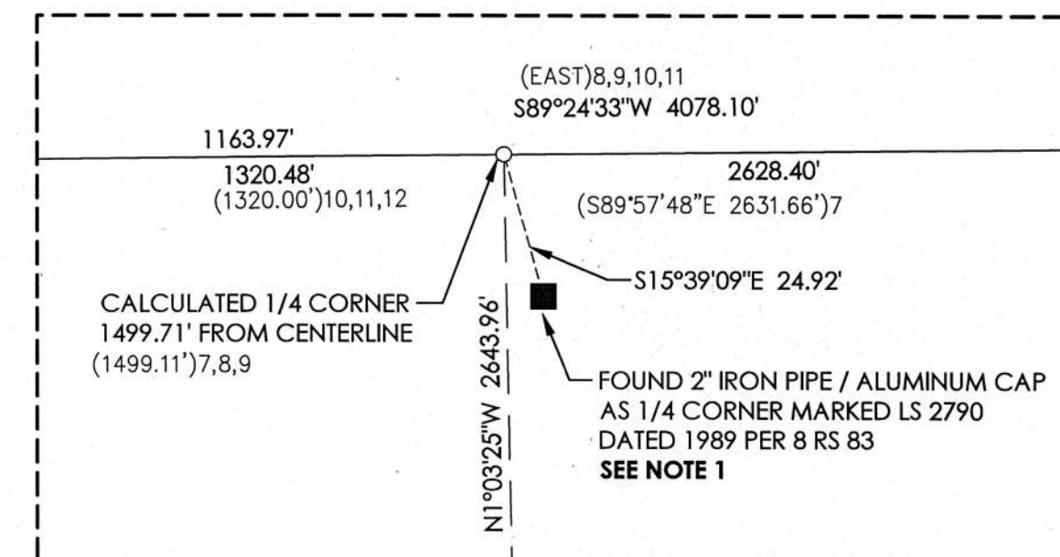
DETAIL 5 1"=30'
