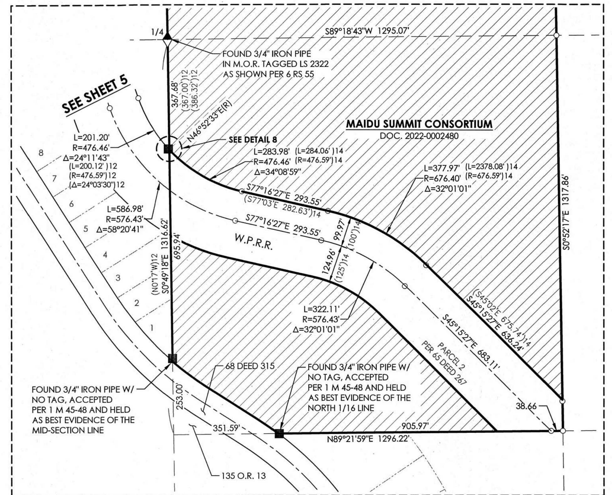
DETAIL 7 1"=200'
