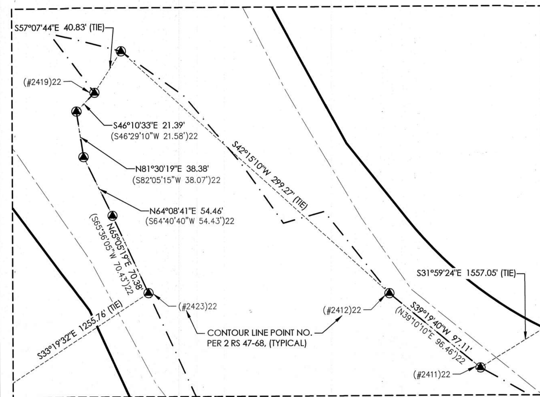
DETAIL 10
