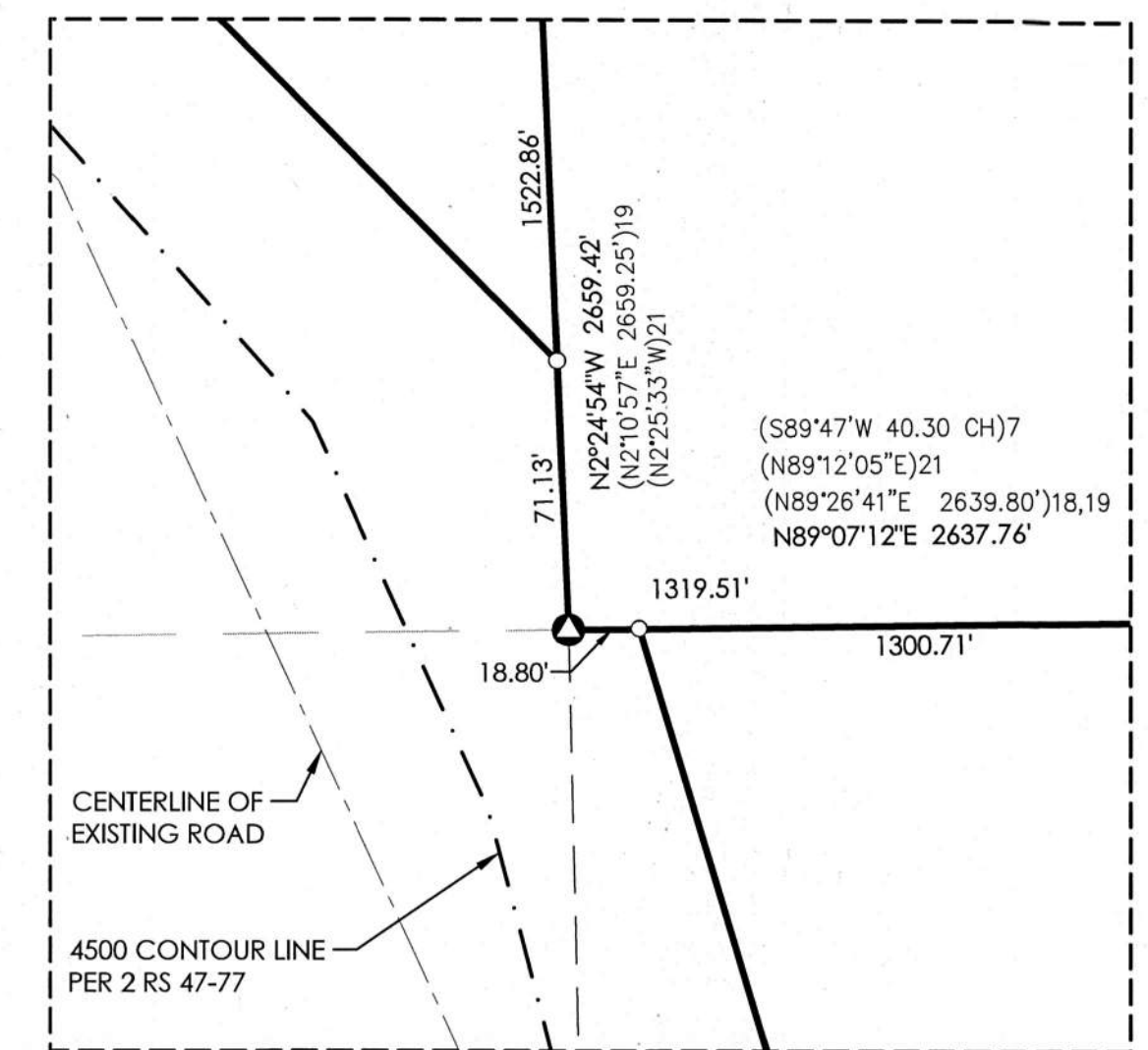
DETAIL 9 1"=50'
