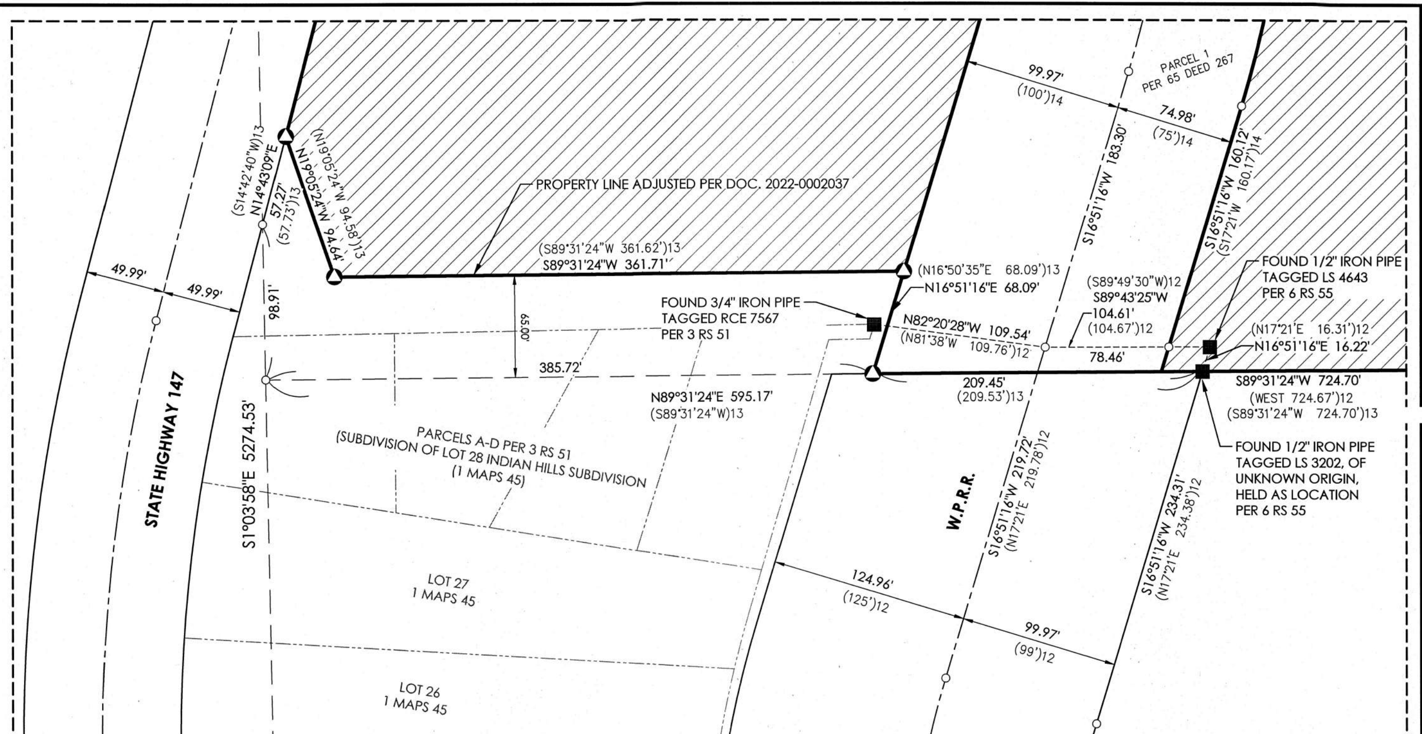
DETAIL 6 1"=60'
