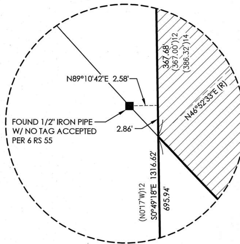
DETAIL 8 1"=5'
