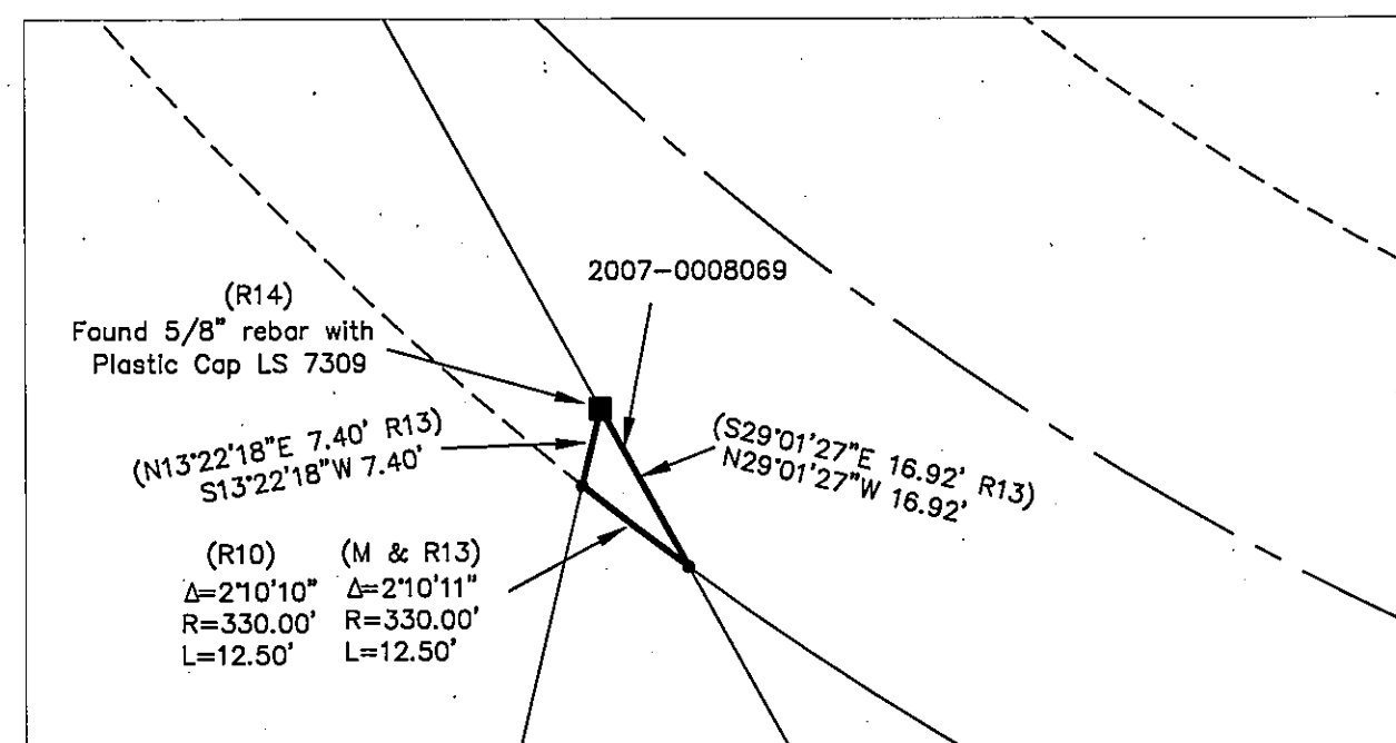
Detail "C-1"
