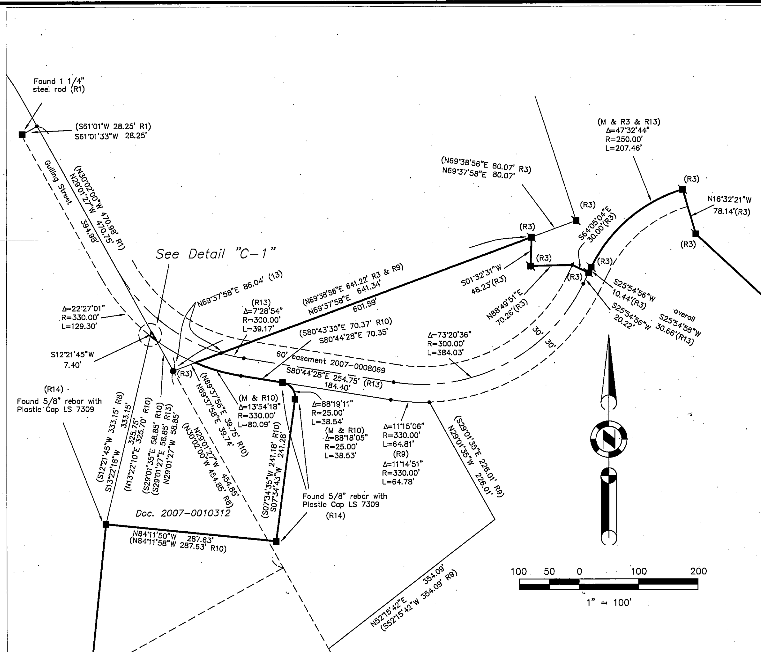
Detail "C"
