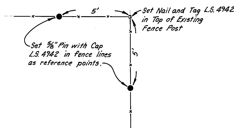
TYPICAL FENCE CORNER MONUMENTATION
