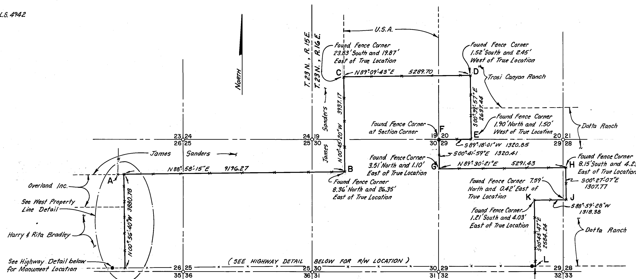
FENCE LINE BOUNDARY
