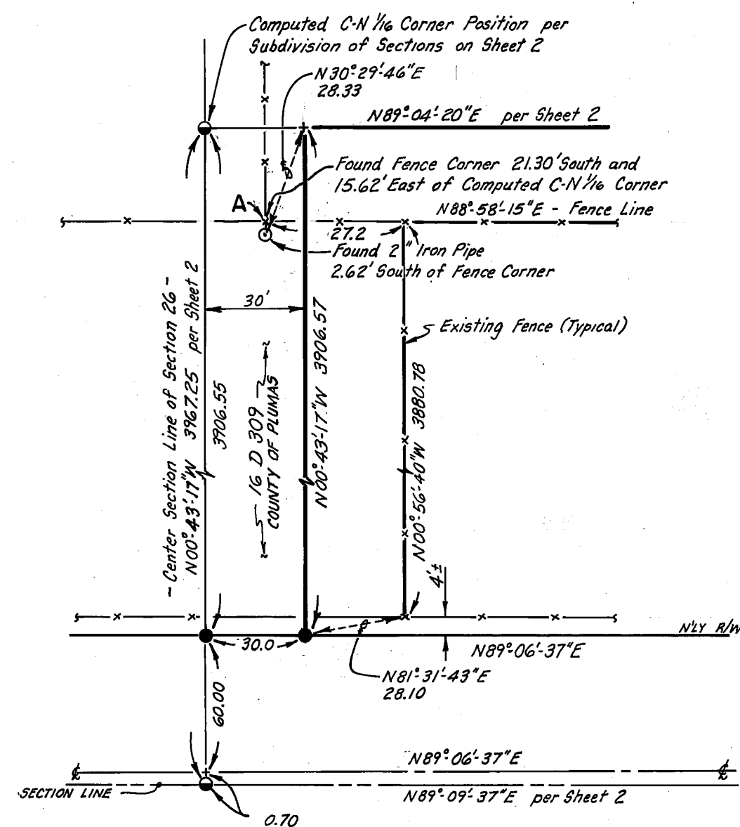
WEST PROPERTY LINE DETAIL
