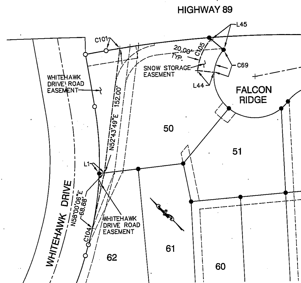
DETAIL A SCALE: 1"=60'
