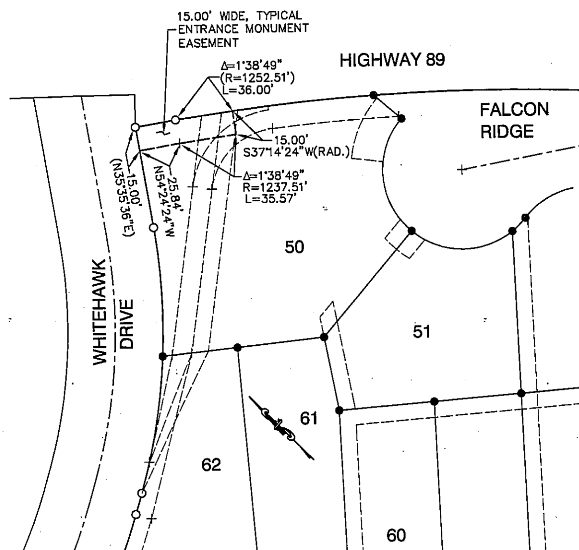
DETAIL D SCALE: 1"=60'
