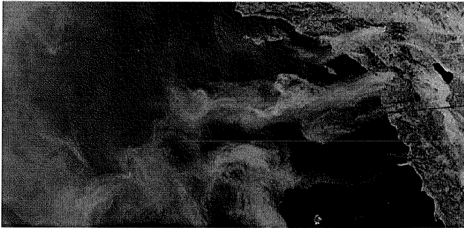
Figure 1 Discrete smoke plumes early in fire's evolution
